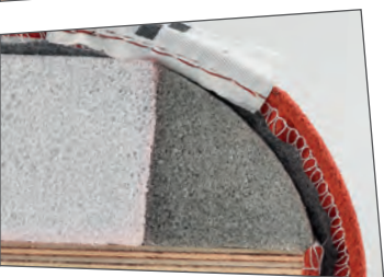
22 | FoamFlex light, 35 x 70 mm, FoamFlex light, 35 x 70 mm.
